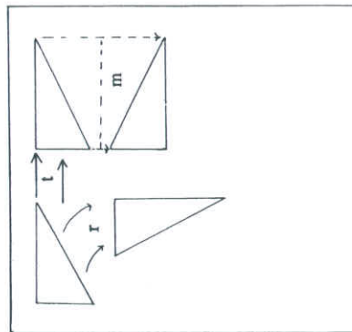
Figure 10. In Euclidean geometry, a translation ( t ), a rotation ( r ) and a mirror reflection ( m ) move a triangle or other shape to a congruent shape.
