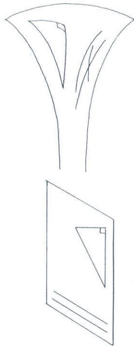
Figure 6. A portion of the Euclidean plane with parallel lines and a right triangle.
