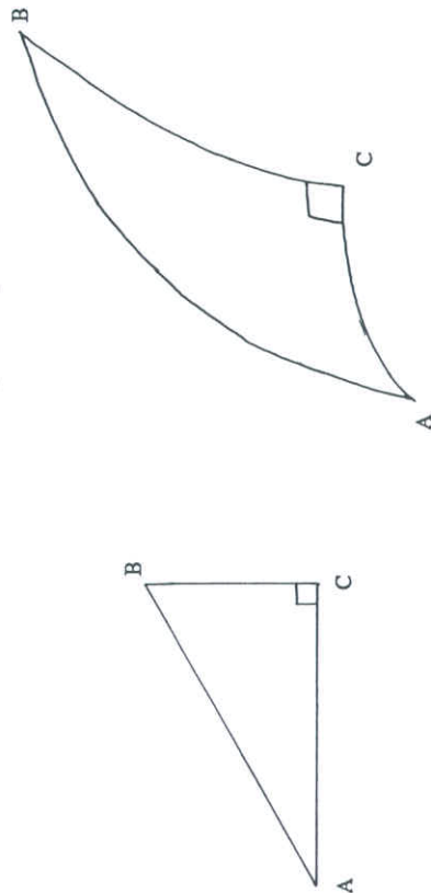
Figure 7. A portion of the hyperbolic plane with lines illustrating the revised postulate and a right triangle.
