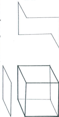
Figure 7. A cube and two possible "substructures."
