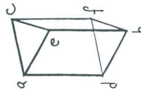
Figure 5. A triangular prism.
