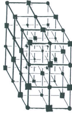
Figure 9. The structure of a salt crystal. The squares represent sodium ions and circles represent chlorine ions.
