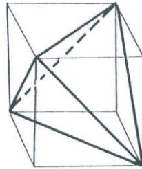
Figure 8. A triangular pyramid as a substructure of a cube.
