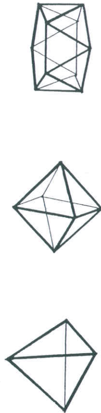
Figure 6. One-point homogeneous figures.
